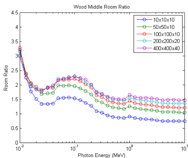
Figure 4-4-15: Surface contamination of wood for middle of the room position
