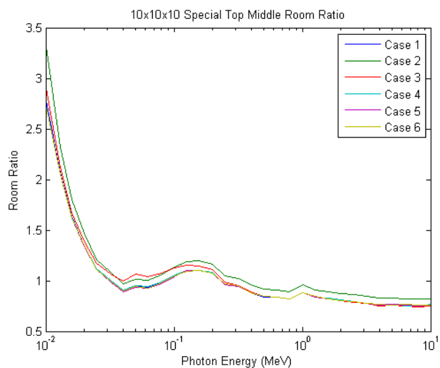
Figure 4-45: Special cases top middle room tally for 10x10x10 room with surface contamination
