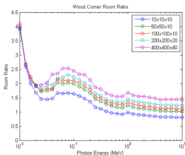
Figure 4-4-14: Surface contamination of wood for corner of the room position
