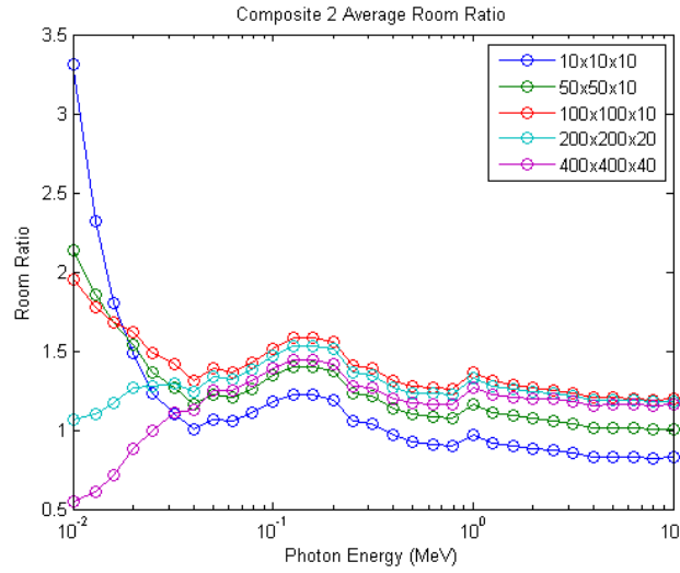
Figure 4-30: Composite 2 average room ratios for all room dimensions with surface contamination
