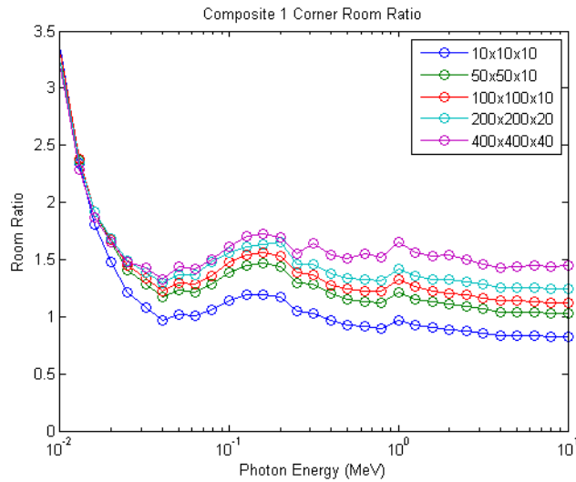
Figure 4-24: Composite 1 corner room ratios for all room dimensions with surface contamination
