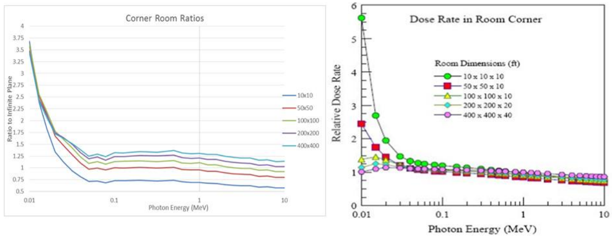
Figure 3-4: Comparison of Corner Room Ratios (Left - MCNP, Right- Point Kernel)
