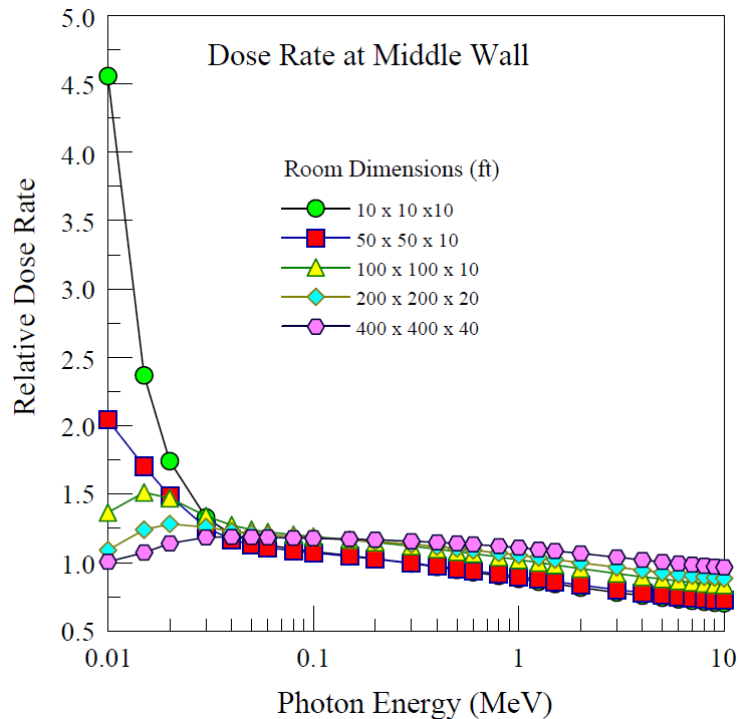
Figure 2-10: Relative dose rate at middle of wall location in rooms of various sizes [7]
