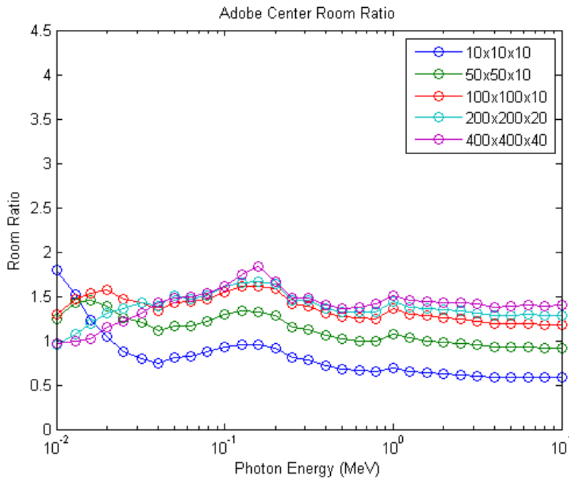
Figure 4-9: Surface contamination of adobe for center of the room position
