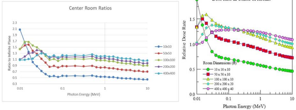
Figure 3-3: Comparison of Center Room Ratios (Left-MCNP, Right-Point Kernel)
