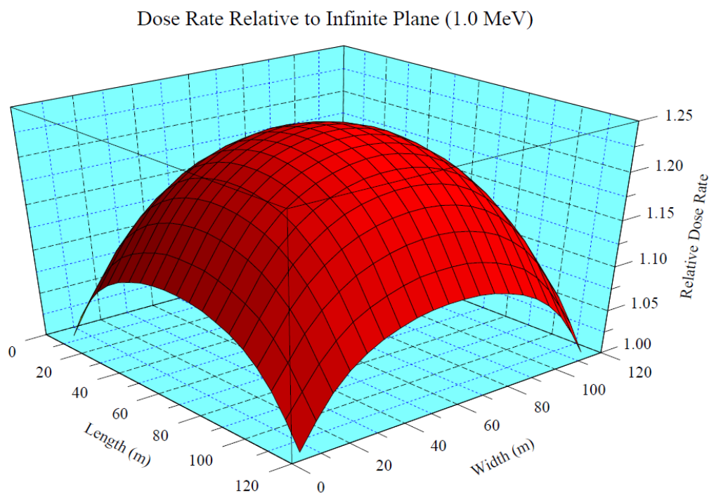
Figure 2-6: Photon dose rate inside large room (400 x 400 x 40 ft) for a 1.0 MeV source [7]
